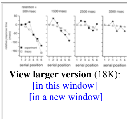
Figure 10. Data from Forrin and Cunningham (1973) + , showing that short-term repetition priming can explain serial position effects. The shorter the delay between presentation of list items and the probe ( t_{\text{retention}} ), the faster the RT (recency), as shown by the solid lines . By modeling the priming by a simple exponential (Fig. 11), recency is fit reasonably well ( broken lines ). Best fit (least mean square): \tau_{\text{prime}} = 1181 msec and \alpha = 250 msec. Response times are plotted relative to serial position 1.
